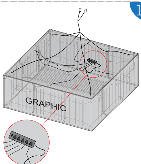
Plug power lines in
