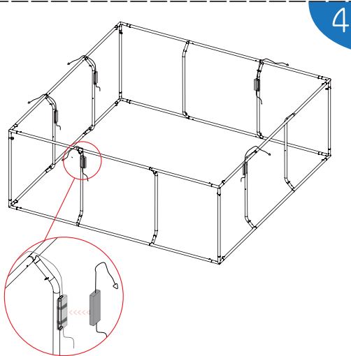
Fix transformers on the frame
