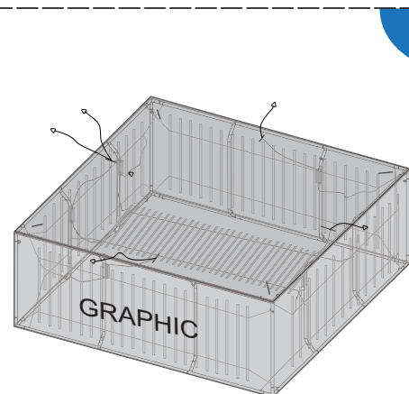
Assemble other else lights as the same label number. (Remark: LED lights should face inside, and power lines are upward.)
