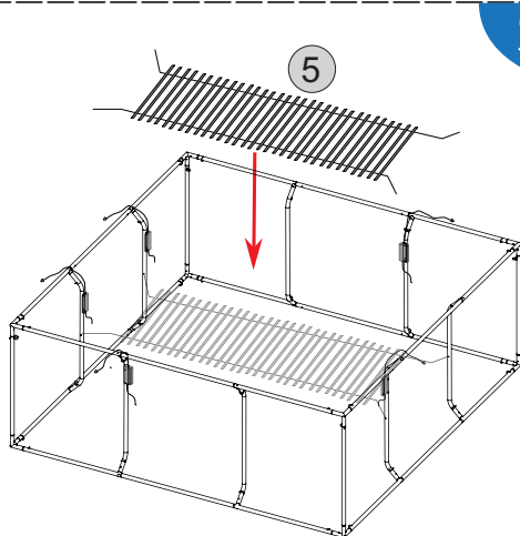
Assemble No.5 LED light first. (Remark: No.5 LED light should face down, and power line should face the side with two transformers.)
