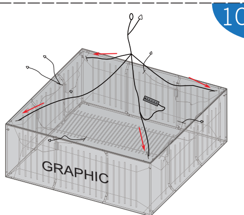
Put the graphic below the frame first, and zip it. (Remark: LED lights should face inside, and power lines are upward.)
